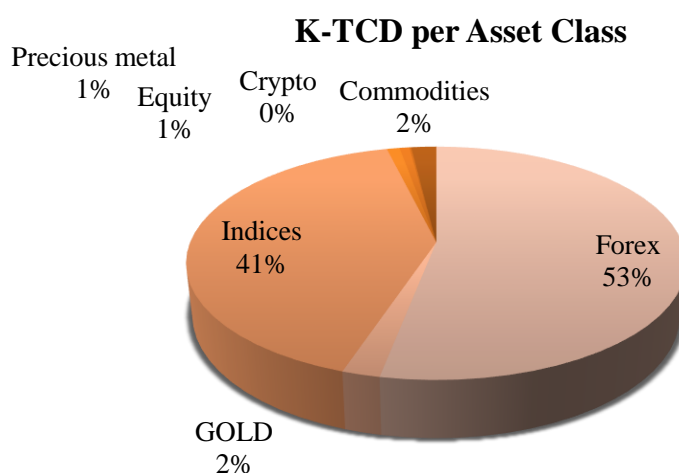
Figure 4: K-TCD Per Asset Class
